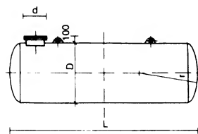
5 Storage tank for heating oil (side view)
